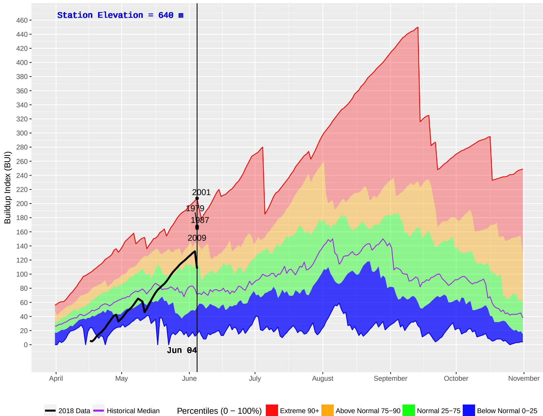
MERRITT HUB (294) : Historical (1978–2016) and Current (2018) Noon Buildup Index (BUI)
