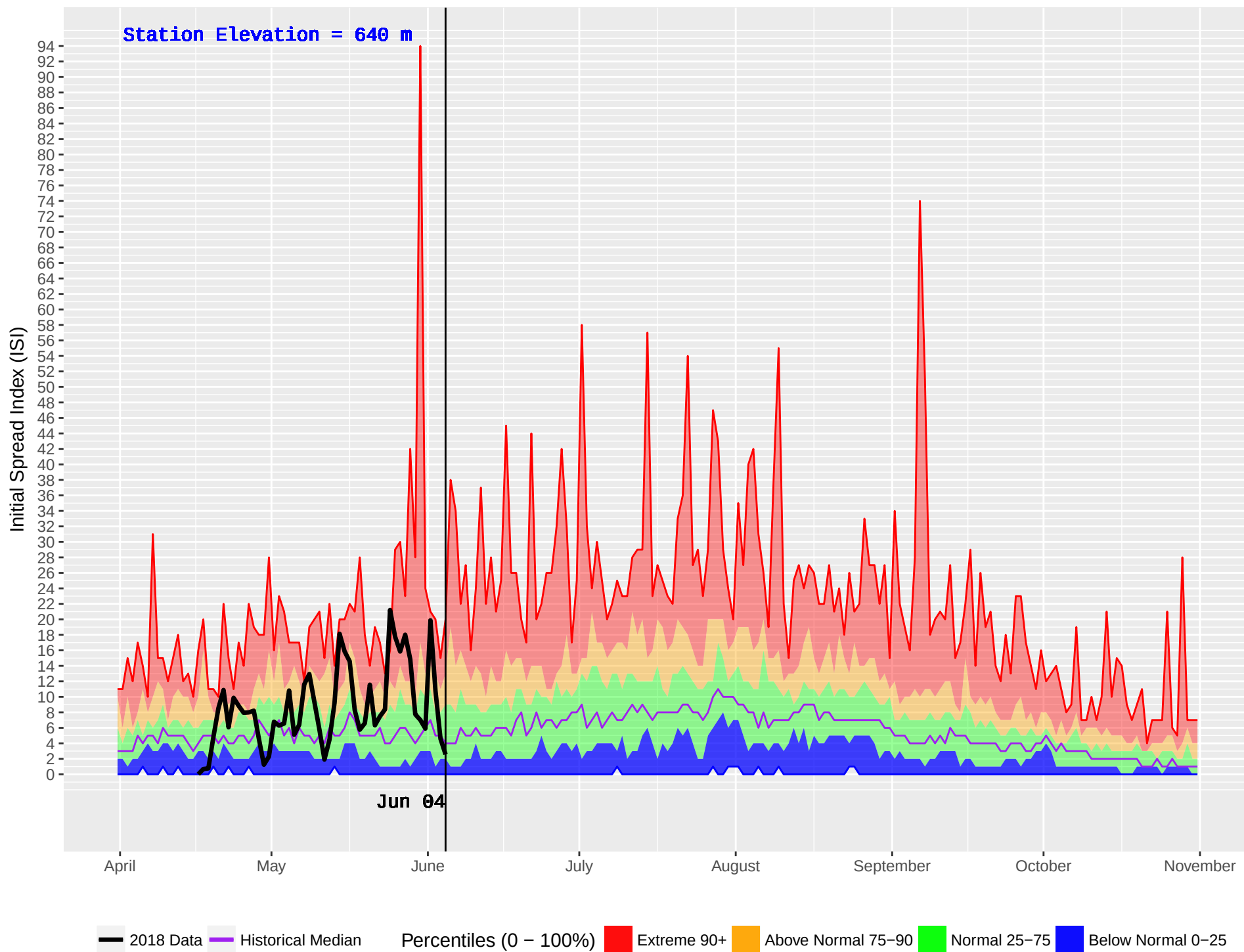
MERRITT HUB (294) : Historical (1978–2016) and Current (2018) Noon Initial Spread Index (ISI)
