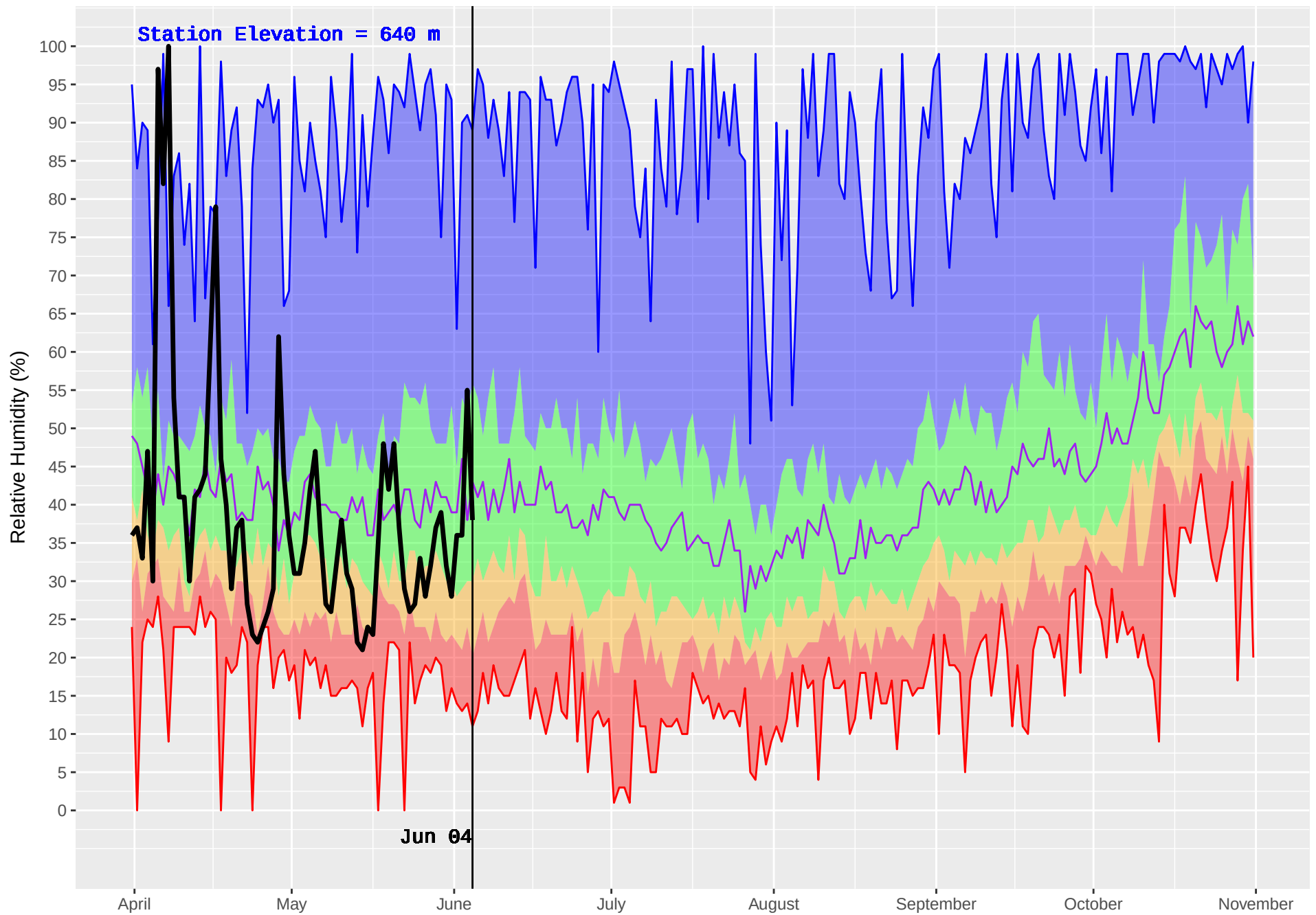
MERRITT HUB (294) : Historical (1978–2016) and Current (2018) Noon Relative Humidity
