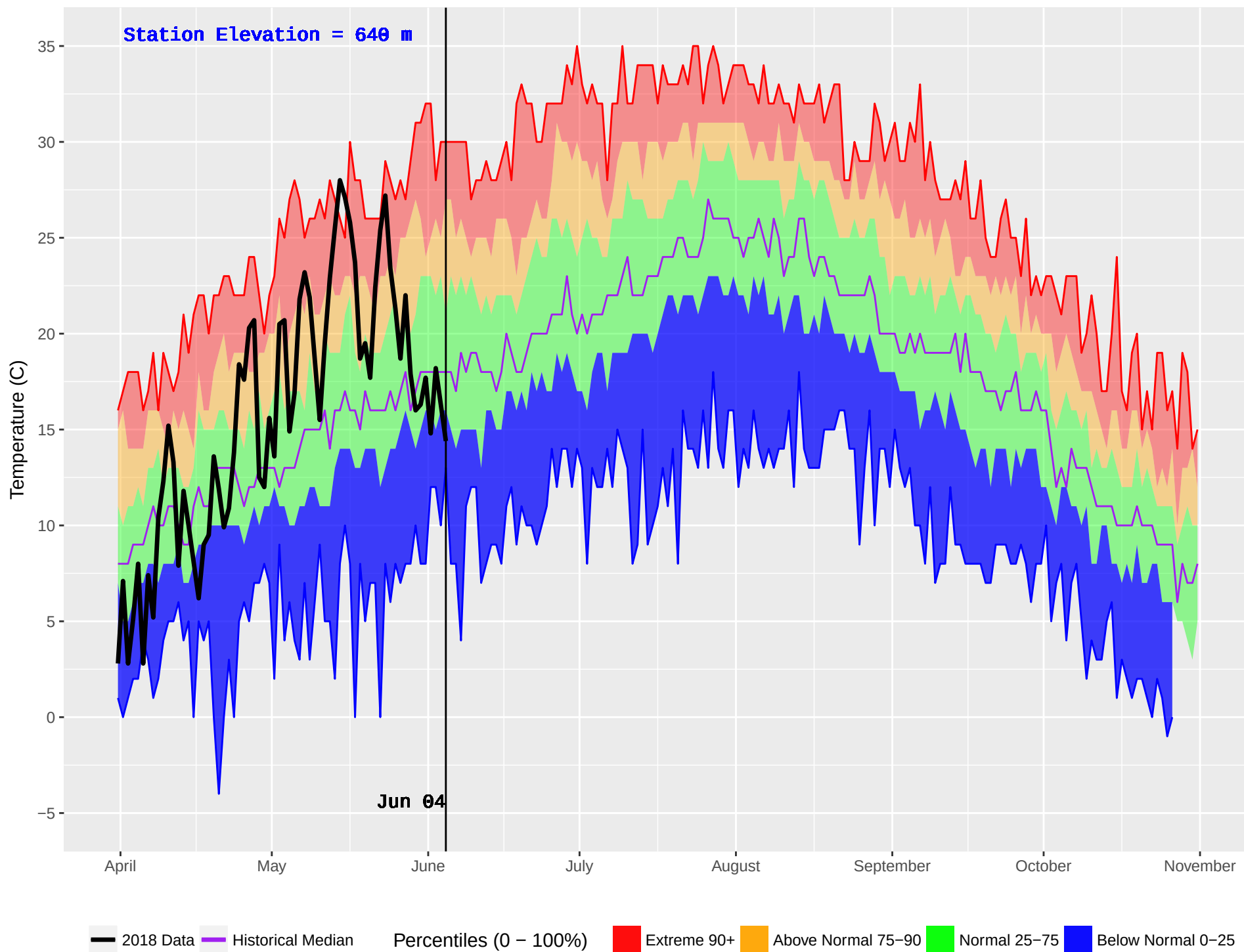
MERRITT HUB (294) : Historical (1978–2016) and Current (2018) Noon Temperature
