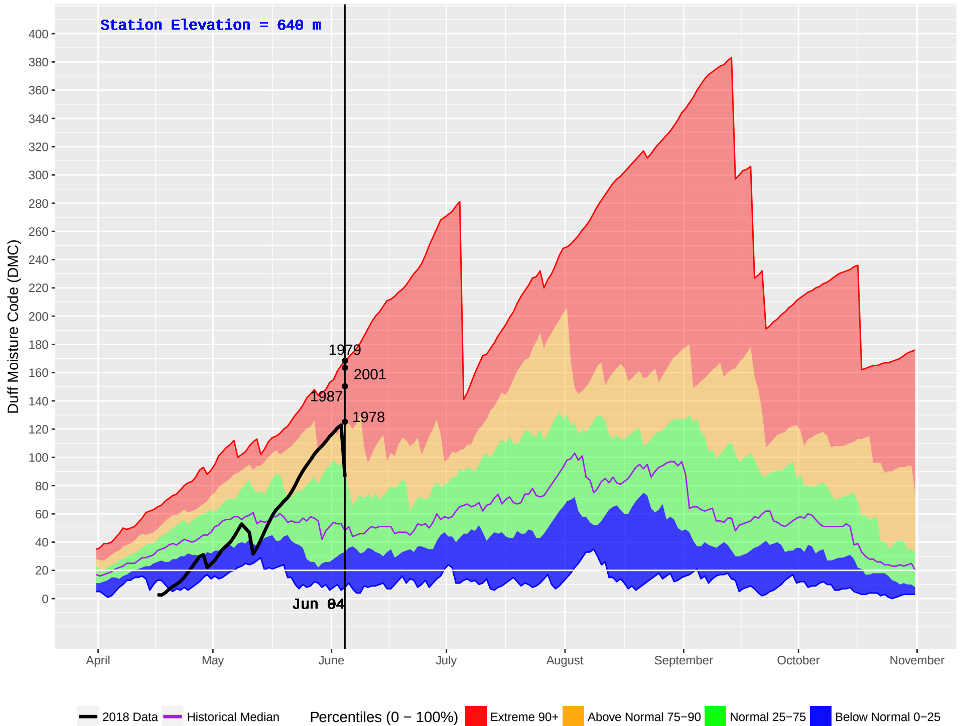
MERRITT HUB (294) : Historical (1978–2016) and Current (2018) Noon Duff Moisture Code (DMC)
